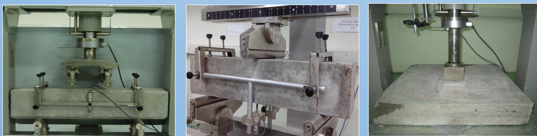
Flexural toughness testing of beams and slabs
